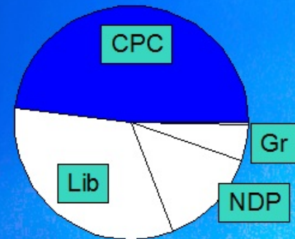
Abbotsford 52% NA
